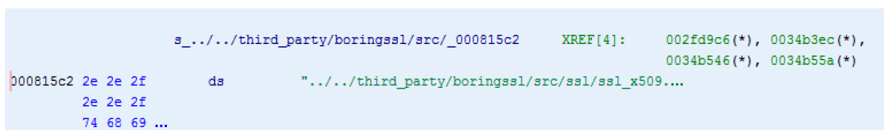
Only 4 xrefs
